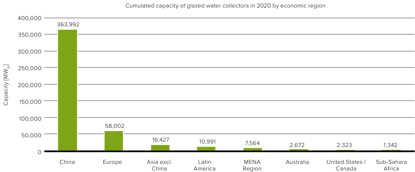
Figure 27: Total capacity of glazed flat plate and evacuated tube collectors in operation by economic region in 2020
