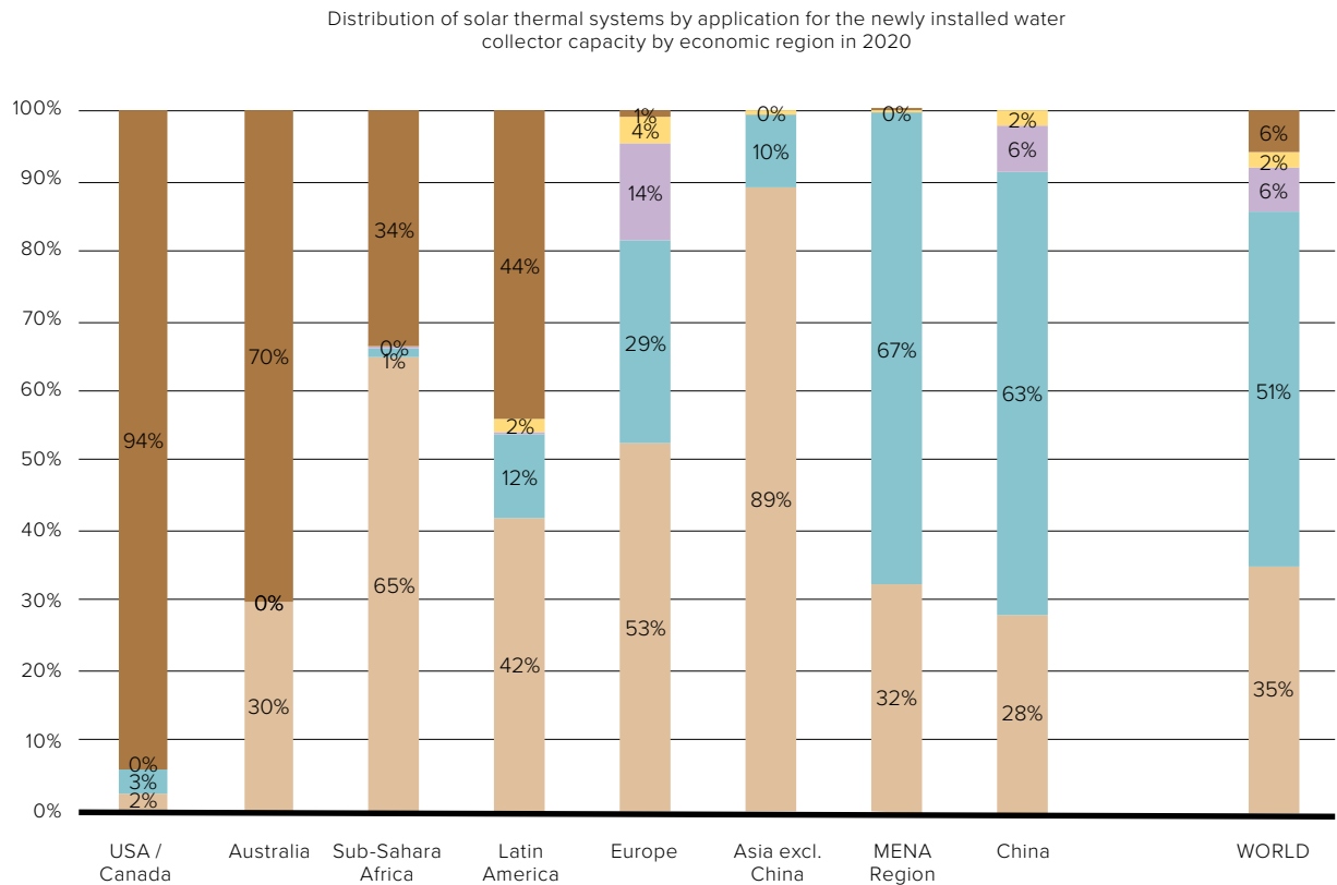
Figure 50: Distribution of solar thermal systems by application for the newly installed water collector capacity by economic region in 2020
